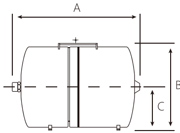
In-line Type
